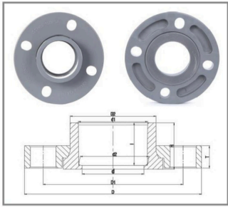
双片式法兰 PP-H --DIN Two-piece Flange PP-H --DIN
