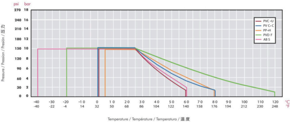
压力/温度图 Pressure/Temperature Graph
